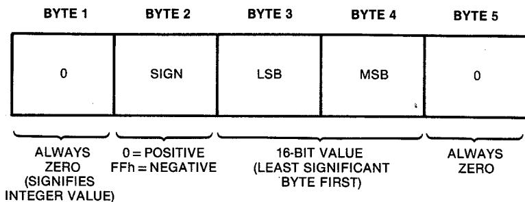
Fig. 3-2. Data structure for an integer value (–65535 to +65535).
